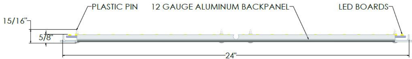
Fig 5: Typical aluminum back panel cross-sectional detail
